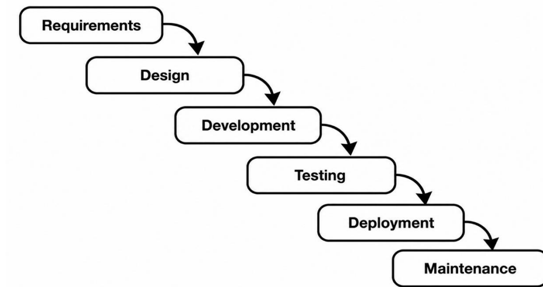
Figure 7.1 : Waterfall Model
